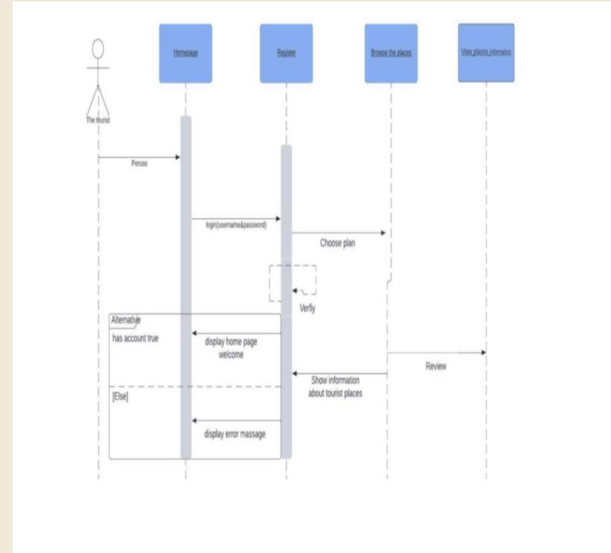
Sequence diagram
