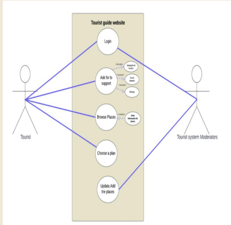
Use-case diagram
